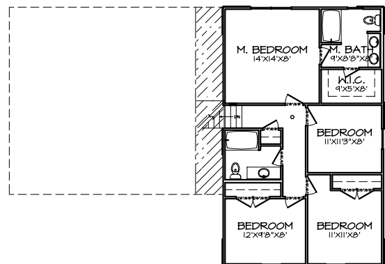
SECOND FLOOR PLAN A-5
