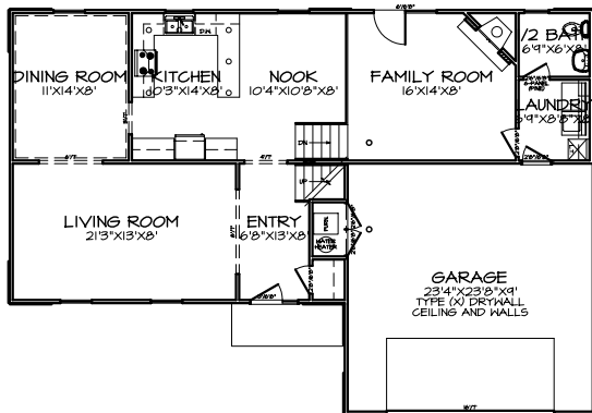
FIRST FLOOR PLAN A-4
